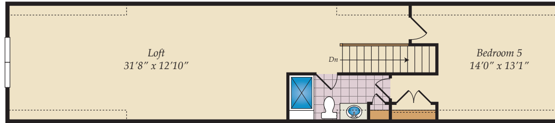
Optional Third Floor
