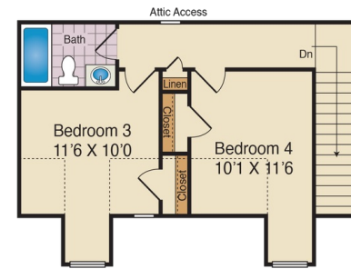
Optional Finished Second Floor
