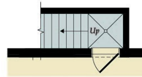
OPT. SINGLE AREAWAY
